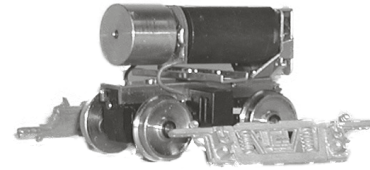
The Power Truck For HO Trolley and Traction Models. 5'7" Wheelbase, 36" wheels. Fully Self Contained, DCC Ready HO-810 Power Truck Only ..... $84.50 HO-811 Power Truck with Trailing Truck ..... $94.50
